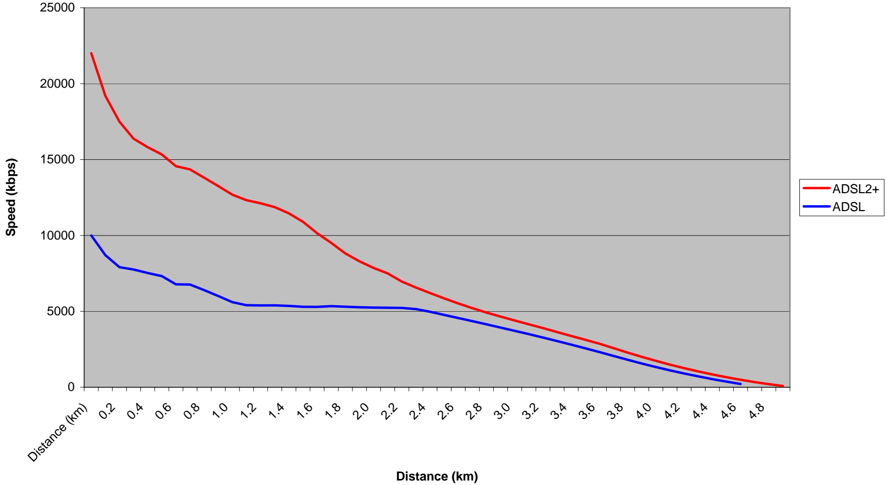
ADSL vs ADSL2+ Performance Comparison Downstream (Assume 0.4 PIUT Cable)
